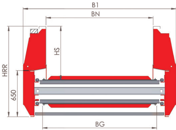
Cross-section of ascending part
