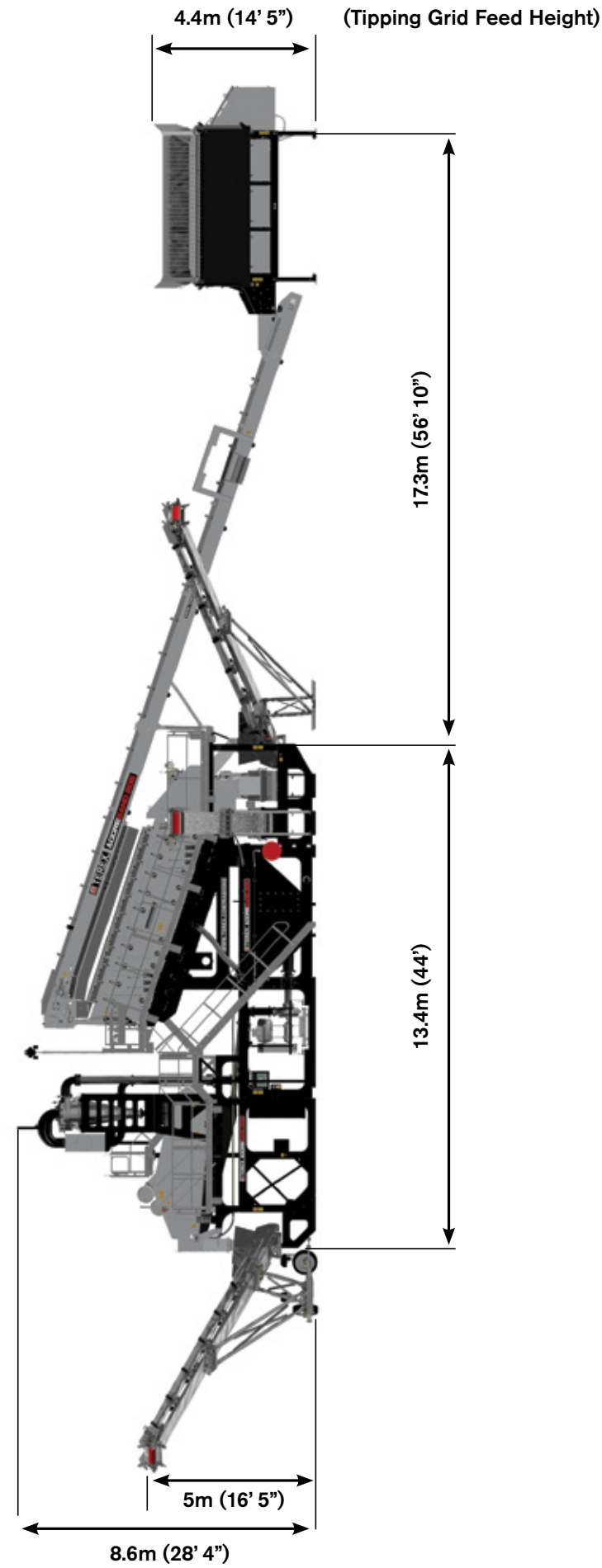
AGGRESAND™ 206 WORKING DIMENSIONS (WITH FEED SYSTEM) HIGH CAPACITY SAND PLANT
